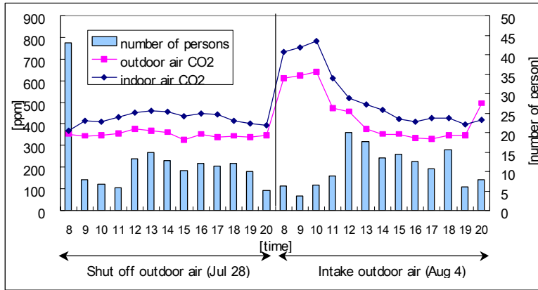
Figure F : Indoor and outdoor CO2 concentrations
