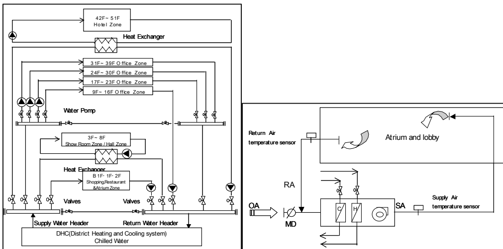
Figure B : HVAC system configurations
