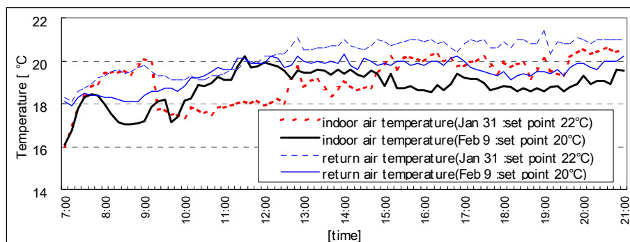
Figure I : Mean atrium temperatures and return air temperatures
