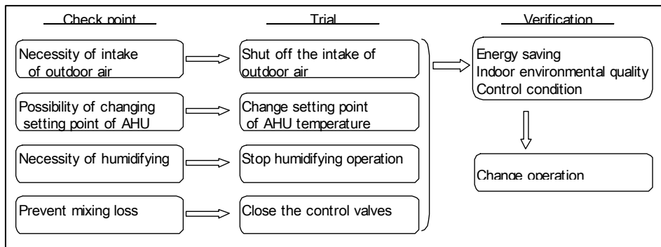
Figure D: Retro-commissioning flows in the atrium and lobby
