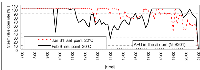
Figure H : Steam control valves open rate
