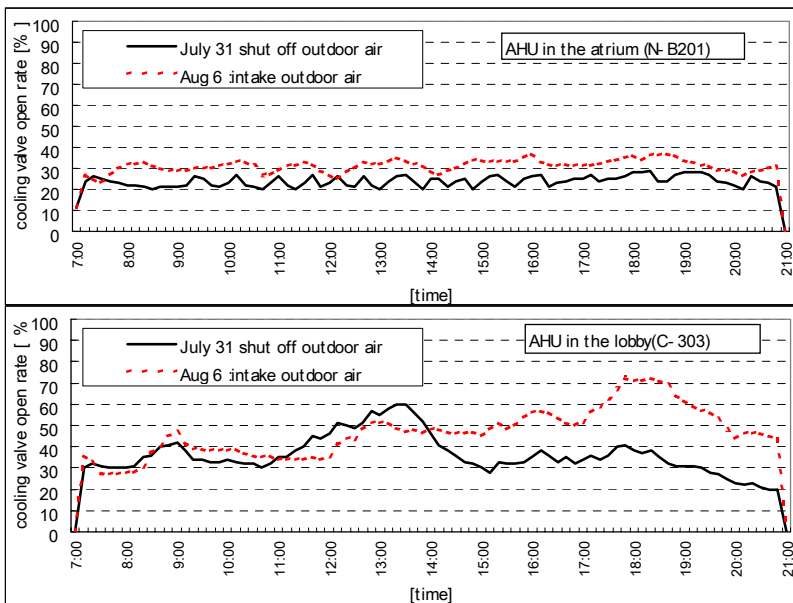
Figure G : Cooling control valves open rate
