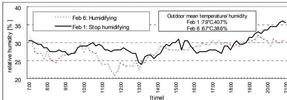
Figure J : Indoor relative humidity measured with and without humidification
