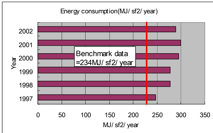
Figure A : Energy consumption for six years
