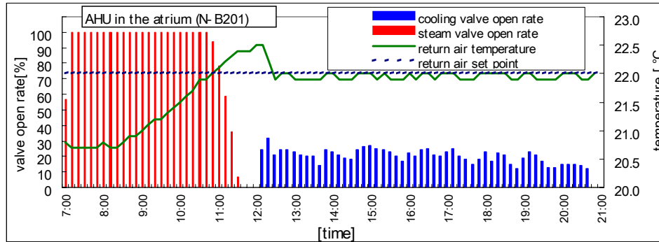
Figure K : Cooling and steam control valve open rate
